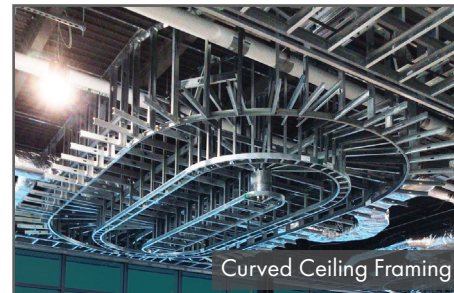
Prefabricated Curved Boxbeams
