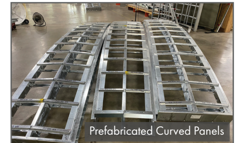
Curved Stud Wall Framing
